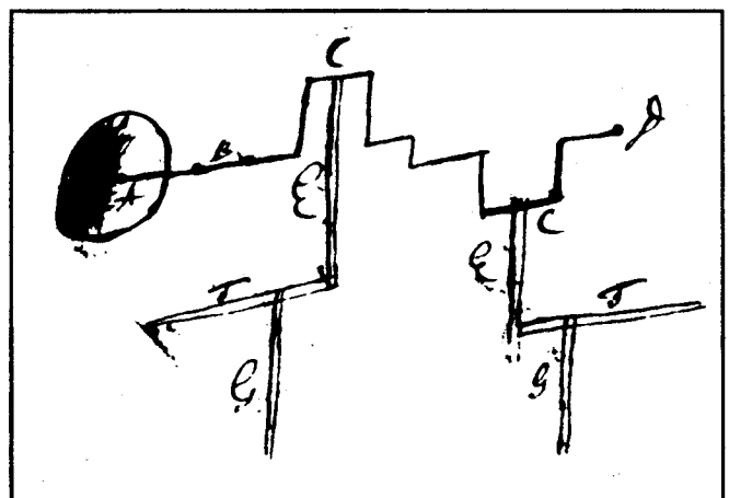
Fig 2. Details of the western pumping wheel at the North Molton Copper Mine, 1725; from Kahlmèter's journal.
