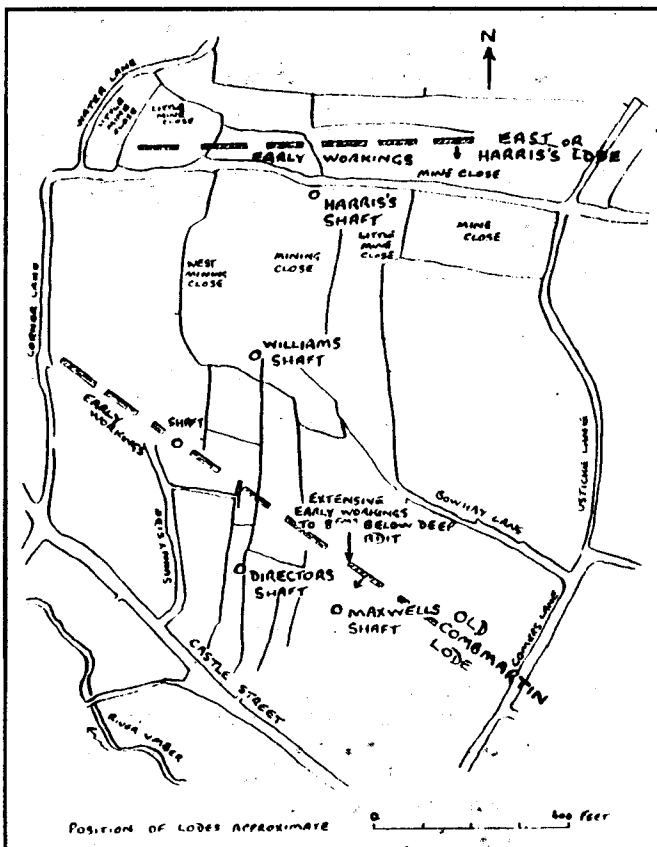
Fig 1. Workings east of the church at Combe Martin, showing some of the principal 19th century shafts.
