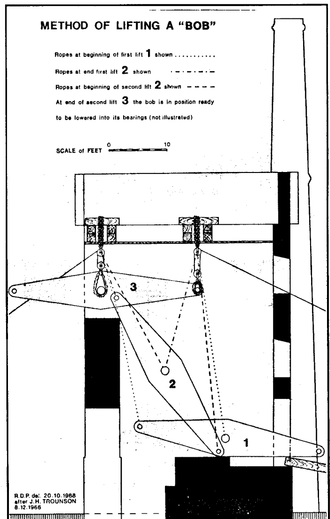
Fig. 4. When erecting an engine the bob was lifted first using tackle suspended from temporary wooden lifting girders, carried on the side walls of the house. The cylinder came in by the same method.
