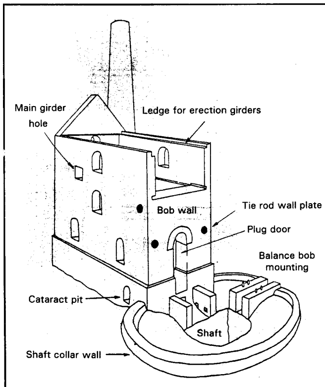
Fig. 3. Isometric view of a pumping engine house, showing external features.
