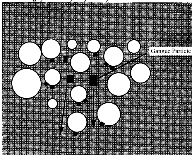
The drainage function of the froth layer.
